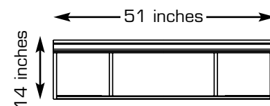
919-590 STORAGE BRIDGE
