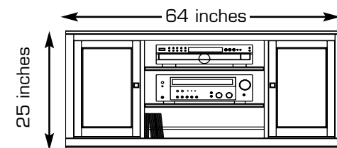
920-583 64" ENTERTAINMENT CENTER
